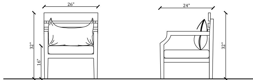
SINGLE SEATER SOFA FRONT VIEW
